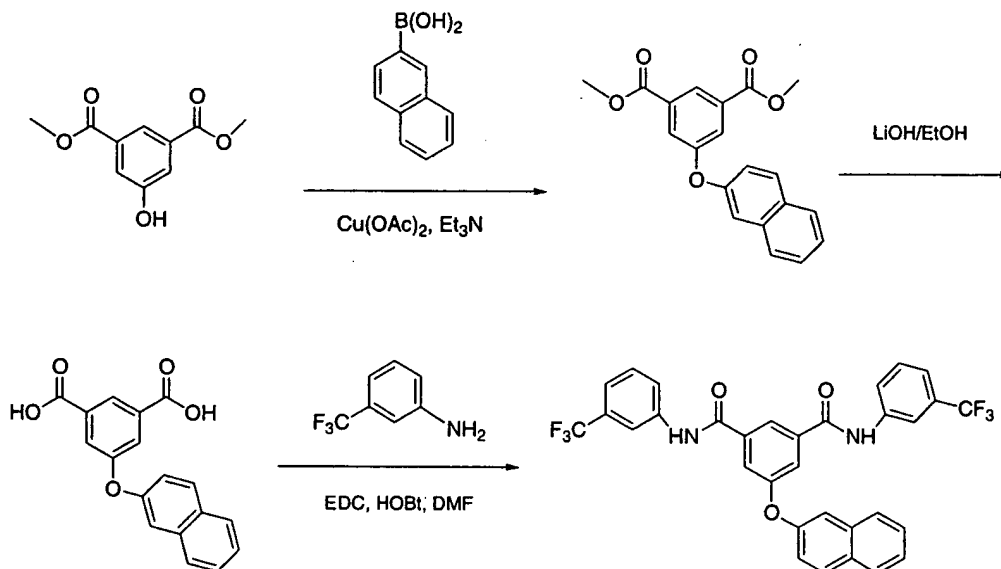
Scheme I-D
